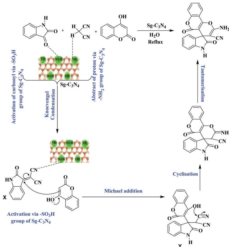
Scheme 3 The probable mechanistic pathway for the production of spiro-pyrano chromens.
