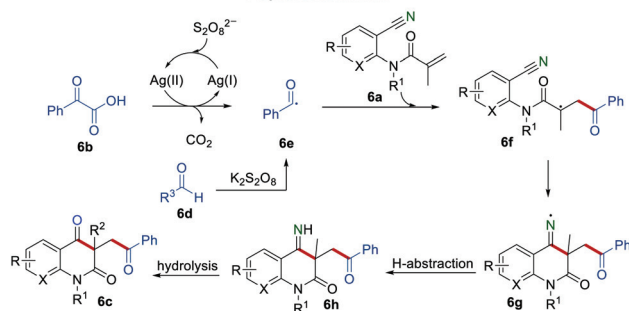
Scheme 6 The construction of the carbonyl-containing quinoline-2,4-diones.
