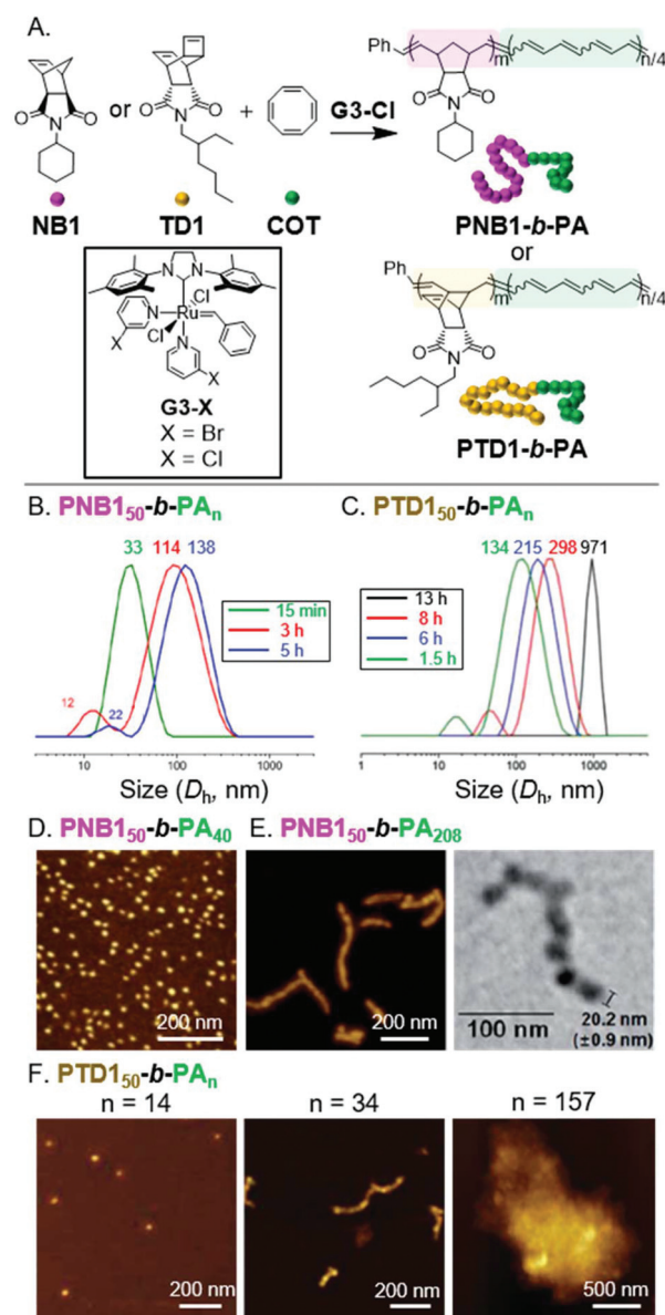
Fig. 2 (A) Synthesis of PA-based BCPs. (B) DLS measurements of aliquots from the polymerization solution of \text{PNB}_{150}\text{-}b\text{-PA}_n . Times are after COT addition. Numbers above the peaks correspond to the average hydrodynamic diameter ( D_{\text{h}} , with units of nm). Adapted from ref. 37 with permission from the Royal Society of Chemistry, copyright 2014. (C) DLS measurements of aliquots from the polymerization solution of \text{PTD}_{150}\text{-}b\text{-PA}_n . Adapted from ref. 38 with permission from John Wiley and Sons, copyright 2015. (D) AFM (on mica) images of nanospheres from \text{PNB}_{150}\text{-}b\text{-PA}_{40} . Adapted from ref. 16 with permission from American Chemical Society, copyright 2012. (E) AFM (on mica) and TEM (on a carbon-coated copper grid) images of nanocaterpillars from \text{PNB}_{150}\text{-}b\text{-PA}_{208} . Adapted from ref. 37 with permission from the Royal Society of Chemistry, copyright 2014. (F) AFM (on mica) images of the nano/micro-object morphologies for \text{PTD}_{150}\text{-}b\text{-PA}_n . Adapted from ref. 38 with permission from John Wiley and Sons, copyright 2015.
