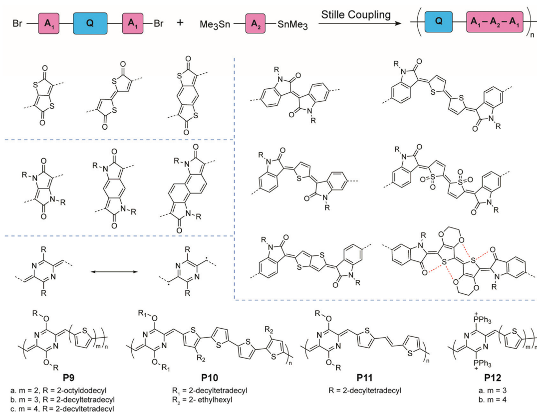
Fig. 6 General synthetic scheme, structural formulae of representative quinoid building blocks, and structures of para -aza-quinoidimethane-derived quinoidal-aromatic alternating copolymers.
