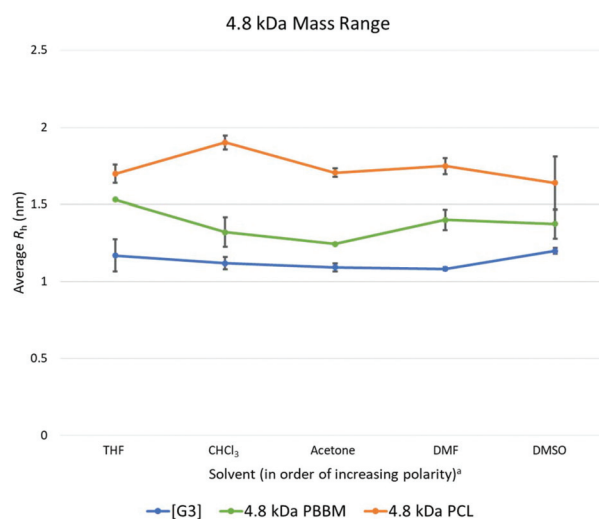
Fig. 7 Calculated average R_h values, from DOSY- ^1\text{H} NMR, for Tetra[G3] Brz 16 , 4.8 kDa PCL, and 4.8 kDa PBBM in all tested solvents. a Solvent polarity values from Reichardt were used to determine order of polarity. 39
