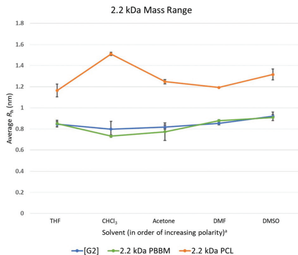
Fig. 6 Calculated average R_h values, from DOSY- ^1\text{H} NMR, for Tetra[G2] Brz 8 , 2.2 kDa PCL, and 2.2 kDa PBBM in all tested solvents. a Solvent polarity values from Reichardt were used to determine order of polarity. 39
