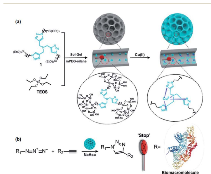
Fig. 45 (a) Cu-TTASi nanoreactors and the detailed coordination relations of Cu II and \text{N}(\text{C}_3\text{N}_3)_3 ligands and (b) Cu I -TTASi-catalyzed CuAAC reactions in the presence of sodium ascorbate. mPEG-silane: PEGylation triethoxysilane; NaAsc: sodium ascorbate. 235 Reproduced with permission. 235 Copyright 2021, American Chemical Society.
