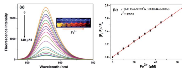
Fig. 3 (a) Fluorescence emission spectra of the N-CDs in pure water ( 0.04\text{ mg mL}^{-1} ) with the different concentrations of \text{Fe}^{3+} (0–140 \mu\text{M} ) under 450 nm excitation. The inset shows the image of the N-CDs in pure water with the increased \text{Fe}^{3+} from left to right under UV lamp irradiation at 365 nm. (b) Linear relationship between [(F_0 - F)/F_0] and the concentrations of \text{Fe}^{3+} , where F_0 and F are the fluorescence intensities of the N-CDs at 556 nm in the absence and presence of \text{Fe}^{3+} , respectively.
