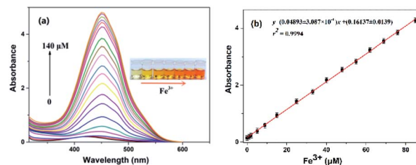
Fig. 2 (a) Absorption spectra of the N-CDs in pure water ( 0.04\text{ mg mL}^{-1} ) with increased concentrations of \text{Fe}^{3+} (0–140 \mu\text{M} ). The inset shows the image of the N-CDs in pure water with the increased \text{Fe}^{3+} from left to right under daylight. (b) Linear relationship between absorbance and the concentration of \text{Fe}^{3+} .
