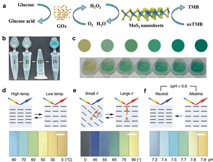
Fig. 22 Colorimetric sensors based on 2D nanomaterials with color-changing capability. (a) Colorimetric glucose sensor from MoS 2 nanosheets and glucose oxidase (GOx). (b) Procedure for glucose detection using the portable test kit, involving initiating the test kit (I), loading the serum sample (II), 60 min incubation at 37 °C (III), and observing the sample colour (IV). (c) Standard colorimetric card of glucose concentration (from left to right: 0, 3, 5, 7, 9, and 12 mM) and images of the hydrogel demonstrating the concentration of the serum glucose in the test kit. (a–c) Reproduced with permission. 423 Copyright 2014, The Royal Society of Chemistry. (d–f) Color changes of 2D TiO 2 dispersion in response to external stimuli. Optical images of the magnetically oriented photonic nanosheet dispersion on changing the temperature (d), angle of an externally applied magnetic flux (e) and the pH value (f). Scale bars are 5 mm in (d–f). (d–f) Reproduced with permission. 427 Copyright 2016, Springer Nature.
