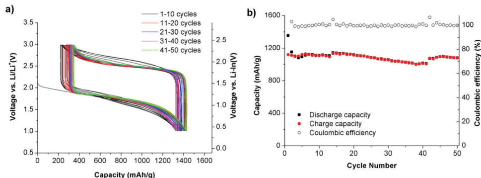
Fig. 20 (a) Discharge–charge curves and (b) discharge/charge capacity and coulombic efficiency of the all-solid-state S/Li_6PS_5Br/In-Li cell up to 50 cycles at room temperature. Image reprinted with permission from ref. 134. https://doi.org/10.1007/s10008-014-2654-1 .
