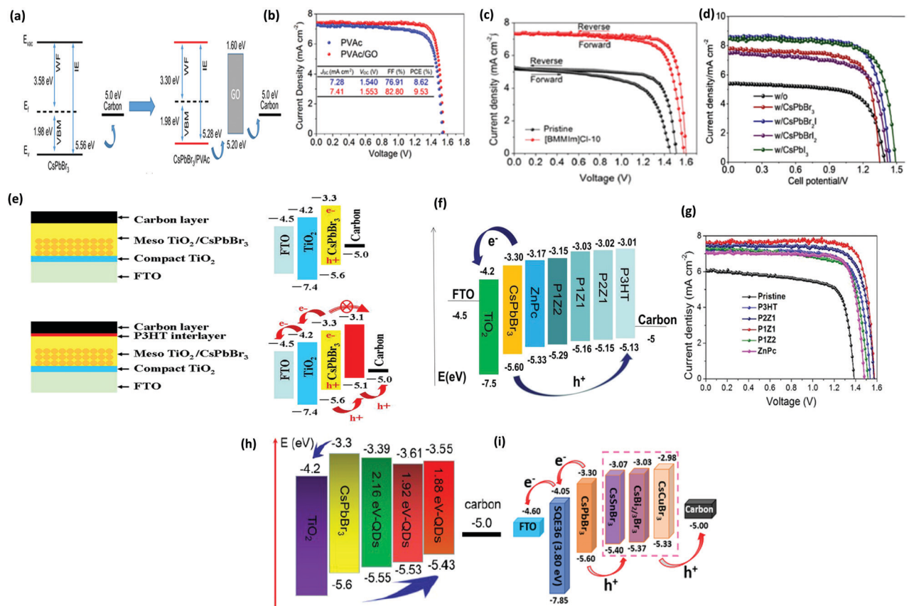
Fig. 20 (a) Schematic illustration of the energy-level relationship of the \text{CsPbBr}_3 layer with PVAc and GO modification. (b) J-V curves of the PVAc-modified \text{CsPbBr}_3 solar cells with and without GO. Reproduced with permission ref. 188. Copyright 2019, American Chemical Society. (c) J-V curves of [BMMIm]Cl ^- incorporated and pure \text{CsPbBr}_3 devices. Reproduced with permission ref. 198. Copyright 2020, American Chemical Society. (d) The corresponding J-V curves of the \text{CsPbBr}_3 solar cells with and without \text{CsPbBr}_{x-1-x} NCs. Reproduced with permission ref. 199. (e) Diagram of the cross-sectional structure and the energy level alignment of the \text{CsPbBr}_3 PSCs without and with the P3HT interlayer. Reproduced with permission ref. 201. Copyright 2019, Elsevier Ltd. (f) Energy level alignment of the materials in the PSC and (g) the photocurrent-voltage ( J-V ) curves of \text{CsPbBr}_3 PSCs with and without HTMs. Reproduced with permission ref. 209. Copyright 2019, The Royal Society of Chemistry. (h) Energy level alignment of each layer in the device. Reproduced with permission ref. 218. Copyright 2018, The Royal Society of Chemistry. (i) Energy level alignment of the PSC with the structure of FTO/SQE/ \text{CsPbBr}_3 / \text{CsMBr}_3 /carbon. Reproduced with permission ref. 219. Copyright 2019, Wiley-VCH.
