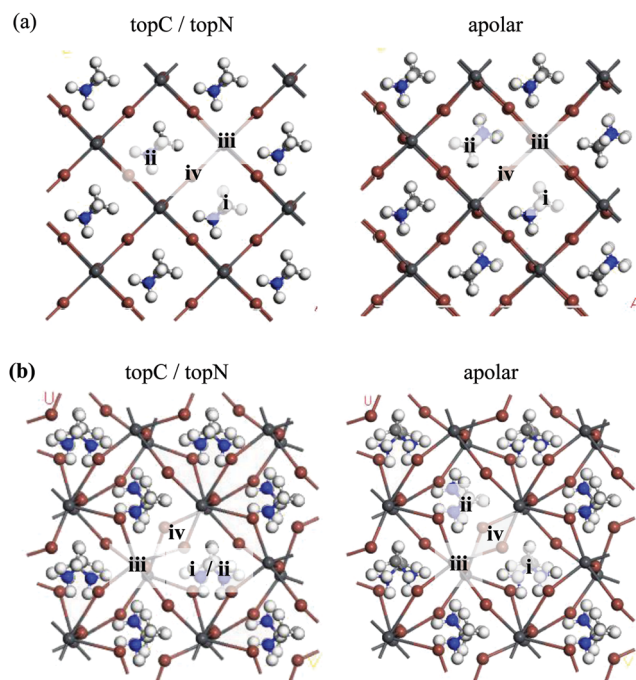
Fig. 3 Position of a fullerene C 60 on (a) cubic and (b) tetragonal MAPbI 3 (001) surfaces with MAI terminations for topC/topN and apolar geometries: (i) aboveN, (ii) above, (iii) above, and (iv) bridge. H, C, N, I, and Pb atoms are represented by the white, light grey, blue, brown, and dark grey spheres, respectively. H, C, N, I, and Pb atoms are represented by the white, light grey, blue, brown, and dark grey spheres, respectively.
