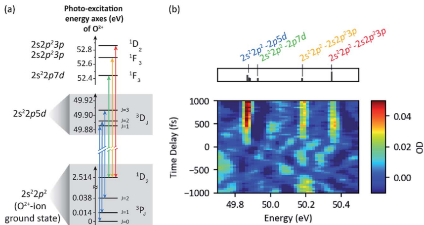
Fig. 8 (a) Level scheme and resonant transitions (indicated by arrows) of the O^{2+} ion—the final atomic dissociation product. (b) XUV-pump XUV-probe transient absorption spectroscopy of molecular oxygen (probe-pulse spectrum). The absorbance is evaluated via a reconstructed reference signal, having excluded all fast oscillating resonance features from the transmitted spectrum by means of a Fourier low-pass filter. Observed absorption lines at positive delays (pump first) correspond to the resonant transitions of the atomic O^{2+} ion indicated in (a).
