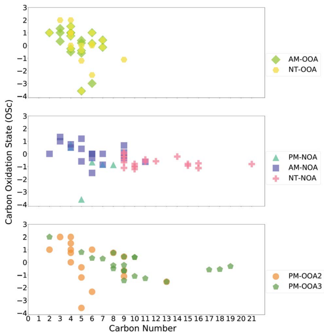
Fig. 4 Oxidation state vs. carbon number plot of top 20 ions most correlated with factors (note: PM-OOA1 shows poor correlation with all ions across the whole time period and thus is not included; its few marker ions during period 2 are discussed in Section 3.4.2).
