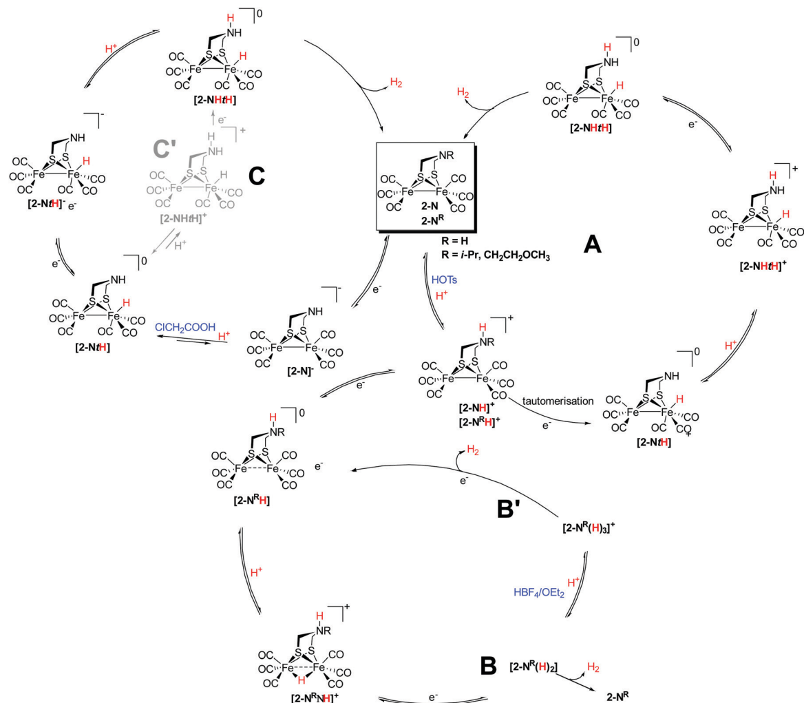
Fig. 99 Catalytic pathways for the proton reduction by \text{Fe}_2(\text{adn})(\text{CO})_6 and \text{Fe}_2(\text{adn}^{\text{R}})(\text{CO})_6 analogues with acids of varying strength.
