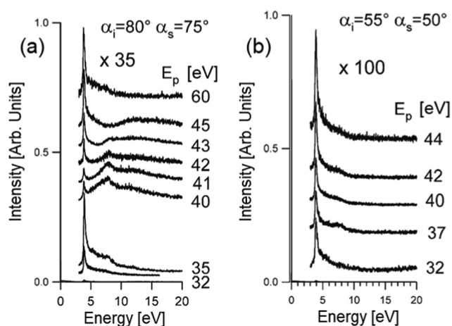
Fig. 8 HREELS spectra of \text{Ag}/\text{Ni}(111) measured in off-specular geometry as a function of the impinging energy for two different conditions (a) \alpha_i = 80^\circ , \alpha_s = 75^\circ ; (b) \alpha_i = 55^\circ , \alpha_s = 50^\circ . Adapted from ref. 101.
