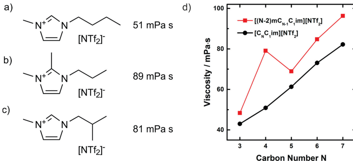
Fig. 21 Viscosities at 25 °C of (a) 268 [C 4 C 1 im][NTf 2 ] - and (b) 271,379 and (c) 268 targeted modifications with the same molecular weight. Slightly lower values for (a) (46 mPa s) and (b) (84 mPa s) were reported in. 380 The dynamic viscosity as a function of the number of carbons in the side chain is shown in (d) for both linear (black curve) and branched (red curve) cations. 268 Reprinted with permission from L. Xue, E. Gurung, G. Tamas, Y. P. Koh, M. Shadeck, S. L. Simon, M. Maroncelli and E. L. Quitevis, J. Chem. Eng. Data , 2016, 61 , 1078–1091. Copyright 2016 American Chemical Society.
