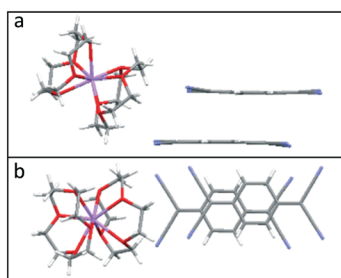
Fig. 6 Side (a) and top (b) views of the (TCNQ) 2 - dimer formed in (12-crown-4) 2 Li(TCNQ) 2 (3).
