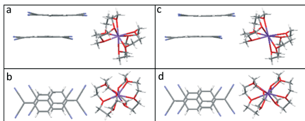
Fig. 7 Side and top views of the (TCNQ) 2 - dimer formed in (12-crown-4) 2 Na(TCNQ) 2 (4) (a and b) and in (12-crown-4) 2 K(TCNQ) 2 (5) (c and d).
