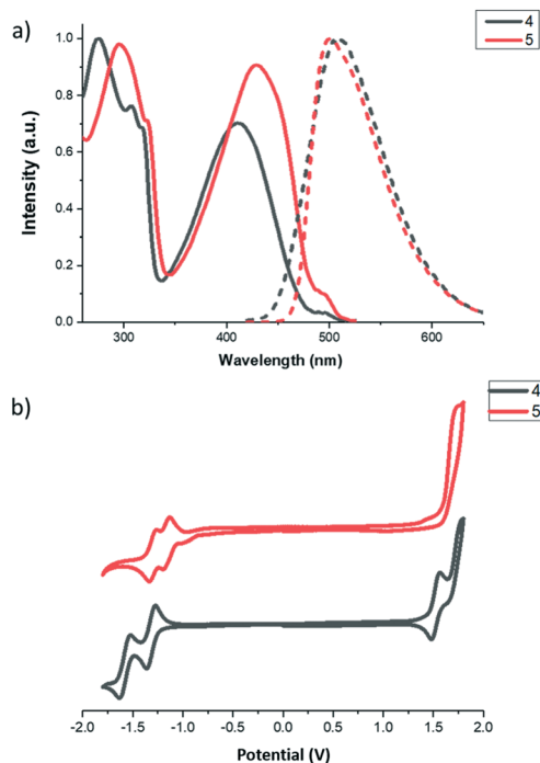
Fig. 1 a) Normalized UV-vis (lines) and fluorescence (dots) spectra of compounds 4–5 in \text{CH}_2\text{Cl}_2 , c = 5 \times 10^{-6} M solutions. b) Cyclic voltammograms of compounds 4–5 at [\text{C}] = 1 \times 10^{-3} M recorded at a scan rate of 100 \text{ mV s}^{-1} in \text{CH}_2\text{Cl}_2/0.1 \text{ M TBAPF}_6 measured versus Ag/AgCl.
