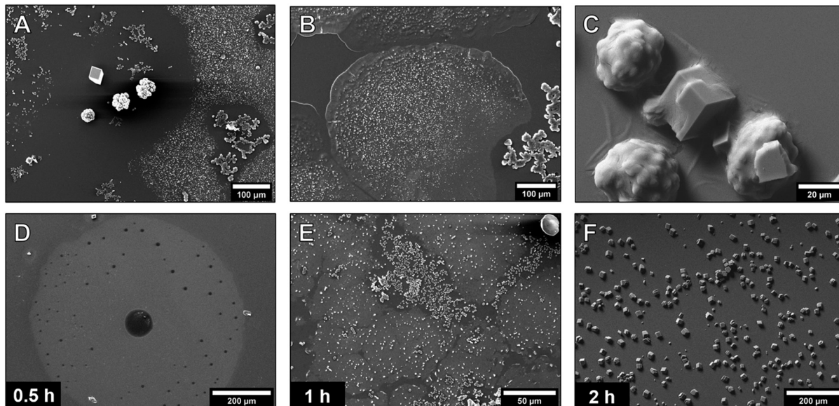
Fig. 3 SEM images for 1 h additive-free gas diffusion experiments using A) 10 mM, B) 20 mM and C) 40 mM \text{CaCl}_2 . A) Different structures are visible on the wafer. No films or smaller particles are visible around larger amorphous or crystalline structures, therefore, likely a dissolution–reprecipitation mechanism occurs. B) In many areas of the wafer, large films with smooth edges were detected. Closer to the center of the spherical structures, smaller particles are visible. C) Calcite and vaterite particles are covered by the film. D)–F) Time-dependent development of the precursor films in the additive-free experiments using 10 mM \text{CaCl}_2 .
