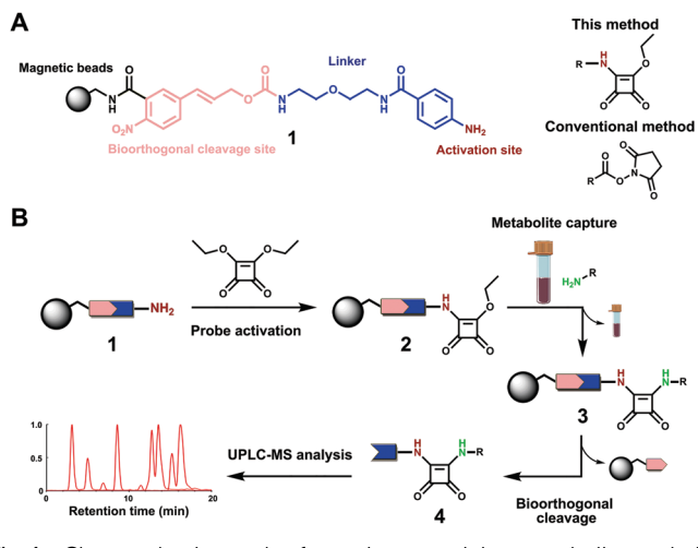
Fig. 1 Chemoselective probe for amine-containing metabolite analysis. (A) Probe design: magnetic beads (black), bioorthogonal cleavage site (pink), linker (blue), and activation site (red). The reactive moiety for amine capturing is a squaramide ester and the conventional moiety an NHS ester. (B) Chemoselective probe treatment workflow that includes a magnetic separation step of 3 from the sample matrix after incubation.
