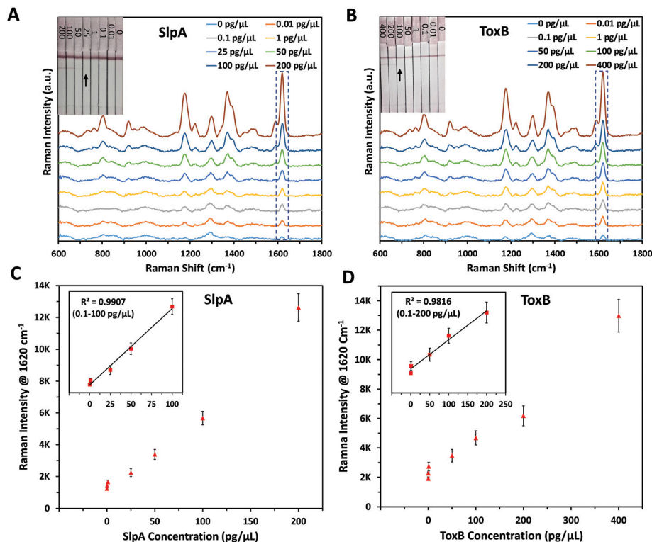
Fig. 2 Raman spectra of (A) SIpA SERS nanotag mixed with different concentrations of SIpA samples (0–200 \mu\text{g L}^{-1} ), (B) ToxB SERS nanotag mixed with different concentrations of ToxB samples (0–400 \mu\text{g L}^{-1} ) on LF strips using handheld Raman spectrometer. The insets show photographic pictures of different biomarkers concentration on their LF strips demonstrating a visual detection limit of 25 \mu\text{g L}^{-1} (SIpA) and 100 \mu\text{g L}^{-1} (ToxB). Corresponding SERS calibration curves for (C) SIpA and (D) ToxB. The insets show the linear dynamic ranges for SIpA (0.1–100 \mu\text{g L}^{-1} ) and ToxB (0.1–200 \mu\text{g L}^{-1} ), respectively. Error bars indicate standard deviations from three measurements. All the SERS measurements were carried out using a handheld Raman spectrometer equipped with a 638 nm laser excitation source at 5 mW laser power with an acquisition time of 0.5 s at ORS mode.
