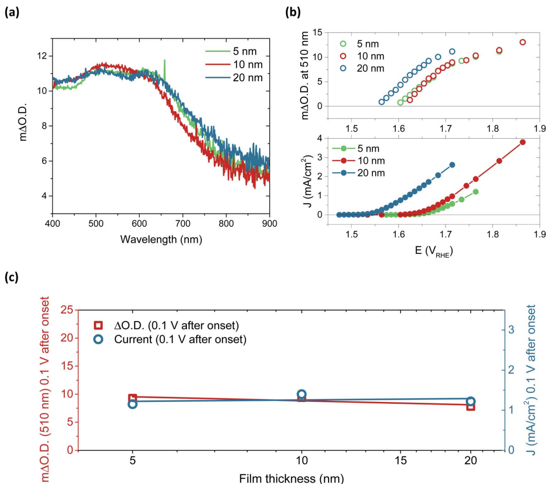
Fig. 3 (a) Spectroelectrochemistry data applying 0.1 V beyond the catalytic onset to ensure each sample is examined under the same catalytic regime (this equates to 1.74 V_{\text{RHE}} for 5 and 10 nm, and 1.65 V_{\text{RHE}} for the 20 nm sample). (b) The change in absorption at 510 nm for each film thickness as a function of applied potential over catalytic range (top), and the corresponding steady-state current obtained simultaneously from the spectroelectrochemistry measurement (bottom) in 0.1 M KOH. In both (a) and (b), 5 nm (green), 10 nm (red), and 20 nm (blue) are shown. (c) The catalytic current and optical density at 510 nm and 0.1 V after current onset against film thickness, revealing no increase in the population of accumulated species with thickness.
