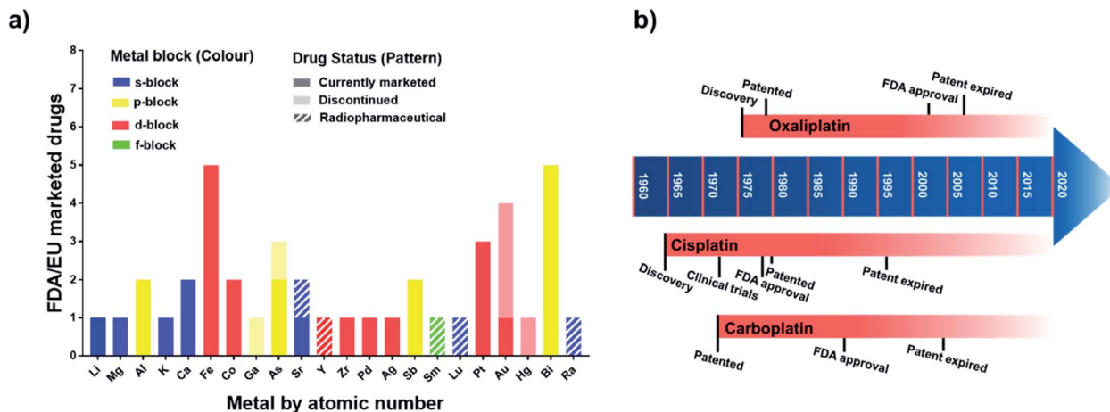
Fig. 1 (a) Metalloids approved in US and/or EU countries classified by metal centre. Different formulations of the same active ingredient are not included, nor are pharmaceuticals where the metal represents only the counter ion. Imaging/diagnostic agents, food supplements, agents used as anaesthetics and in implants are also excluded. A comprehensive list of the agents included is in Table S1.† Remarkably, the total number of clinically-approved metalloids is about half of that for kinase inhibitors, a single class of organic drugs (see https://www.ppu.mrc.ac.uk/list-clinically-approved-kinase-inhibitors ). (b) Timeline describing the development of anticancer drugs cisplatin (Pt1), carboplatin (Pt2) and oxaliplatin (Pt3).
