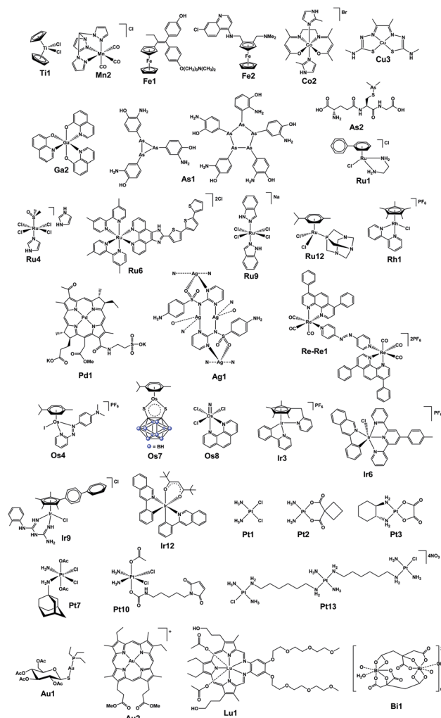
Fig. 2 Structures of selected (candidate) metalloids. Others labelled in the text are in the ESI, Section 6.†
