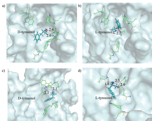
Fig. 3 The representative binding models of D and L -tyrosinol on the outer surface of the (a, b) Poly(D-Trp) and (c, d) Poly(L-Trp) shell. The outer surfaces of Poly(D-/L-Trp) are shown as pale cyan surfaces. D / L -tyrosinol is shown as a ball_and_stick model. The residues stabilizing D and L -tyrosinol by hydrophobic or hydrogen bond interactions are shown as lines. Hydrogen bonds are shown as red dashes and their distances are noted.
