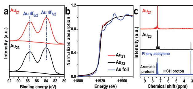
Fig. 5 (a) Au 4f XPS and (b) Au L 3 -edge XANES profiles of \text{Au}_{21}(\text{SR})_{12}(\text{Ph}_2\text{PCH}_2\text{PPh}_2)_2 and \text{Au}_{23}(\text{SR})_{16} . (c) The 1 H NMR spectra of Au-acetylide species.
