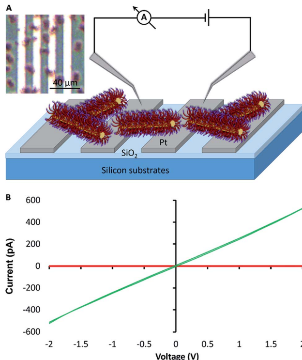
Fig. 5 Fabrication of a simple mesoscopic electrical device. (A) Schematic representation of a simple electrical circuit constructed from bundles of fibre-like terpolymer micelles grown on platinum microband electrodes. (B) I - V measurements of the fibre-like micelles before (red) and after (green) doping with \text{NOBF}_4 . Inset, an optical image of bundles of fibre-like micelles grown from adsorbed seeds on a platinum microband electrode (MBE). Bundles of fibre-like micelles were grown from a high concentration of seeds ( 0.1 \mu\text{g ml}^{-1} , 10 min) and unimer ( 10 \mu\text{l ml}^{-1} , 7 days); they appear as red spots on the platinum MBE in the optical micrograph.
