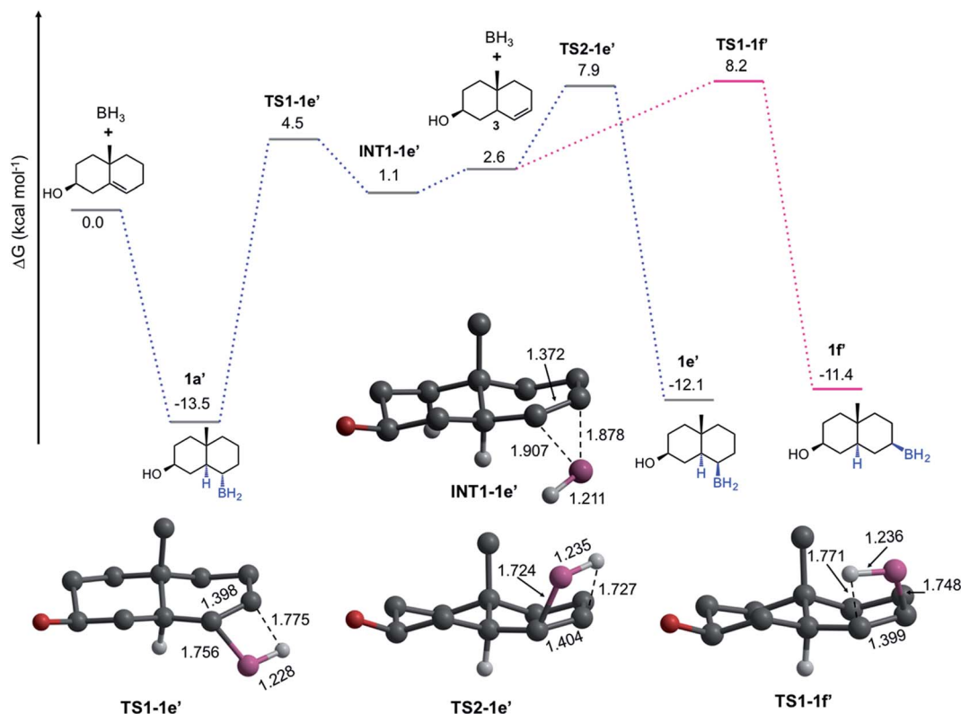
Fig. 4 Gibbs energy profiles (in kcal mol ^{-1} ) for the formation of 1e' and 1f' and transition state structures involved. Bond distances are in Å. In the depicted structures, H atoms are omitted for clarity, except the H atom involved in the hydroboration.
