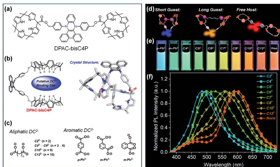
Fig. 6 (a) Chemical and (b) crystal structure of DPAC-bisC4P , as well as (c) chemical structures for various dicarboxylate anionic guests ( DC^{2-} ). (d) Working principle of the fluorescence tuning of DPAC-bisC4P \supset DC^{2-} . (e) Photographs of DPAC-bisC4P \supset DC^{2-} and DPAC-bisC4P in acetonitrile obtained under 365 nm UV light illumination. (f) Normalized photoluminescence (PL) spectra of DPAC-bisC4P in the presence of various linear saturated dicarboxylates at the end of titrations. Reproduced from ref. 104 with permission from the American Chemical Society, Copyright 2019.
