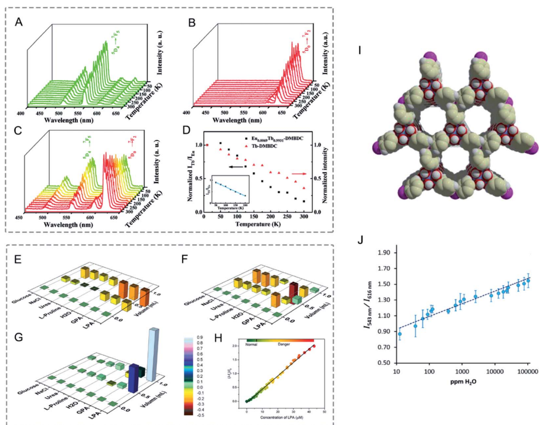
Fig. 15 (A–C) Emission spectra of (A) Tb-DMBDC, (B) Eu-DMBDC, and (C) Eu 0.0069 Tb 0.9931 -DMBDC recorded from 10 and 300 K (excited at 355 nm from the third harmonic of a Nd:YAG laser). (D) Temperature dependence of the integrated intensity ratio of Tb 3+ (545 nm) to Eu 3+ (613 nm) for Eu 0.0069 Tb 0.9931 -DMBDC (black squares), and temperature dependence of the integrated intensity of Tb 3+ (545 nm) for Tb-DMBDC (red triangles). (Inset) Fitted curves of the integrated intensity ratio for Eu 0.0069 Tb 0.9931 -DMBDC from 50 to 200 K. Reproduced with permission from ref. 206. Copyright 2012, American Chemical Society. (E–G) Relative luminescence intensity changes of (E) Tb-ZMOF, (F) Eu-ZMOF, and (G) MZMOF-3 in the presence of different analytes. The intensity change is indicated by the colormap from –0.5 to 0.9. (H) Integrated luminescence intensity changes of MZMOF-3 suspended in MeOH toward 0.03, 0.10, and 0.13 mM LPA. Reproduced with permission from ref. 207. Copyright 2015, American Chemical Society. (I) Chemical Structure of PCM-22. (J) Relative photoemission response ratios obtained upon addition of trace H 2 O to Eu 1 :Tb 5 -PCM-22 pre-soaked in D 2 O showing a linear response. Error bars were obtained from three separate experiments. Reproduced with permission from ref. 208. Copyright 2017, Elsevier.
