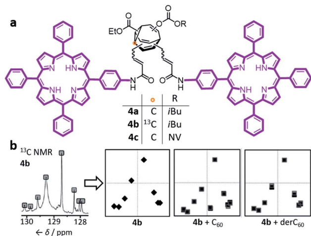
Fig. 4 (a) Bode's bisporphyrin-bullvalene 4 , which was prepared with natural isotopic abundance ( 4a ), enriched in 13 C at one position ( 4b ) of the dynamic C 10 core, and functionalised with a photocleavable group ( 4c ). (b) The complex 13 C NMR spectra of the dynamic mixtures are converted to simplified representations, showing that the 13 C NMR spectrum of a 4b mixture at equilibrium changes in the presence of fullerene guests. NMR data (150 MHz, solutions in CS 2 with 3% CD 2 Cl 2 ) shown for samples of: ( 4b ) 2.8 mM 4b ; ( 4b + C 60 ) 2.8 mM 4b with 2 equiv. C 60 ; ( 4b + derC 60 ) 2.8 mM 4b with 4 equiv. derC 60 . The representations of NMR spectra correspond to two trials overlaid. NV = o -nitroveratryl. Adapted from ref. 7e with permission from The Royal Society of Chemistry.
