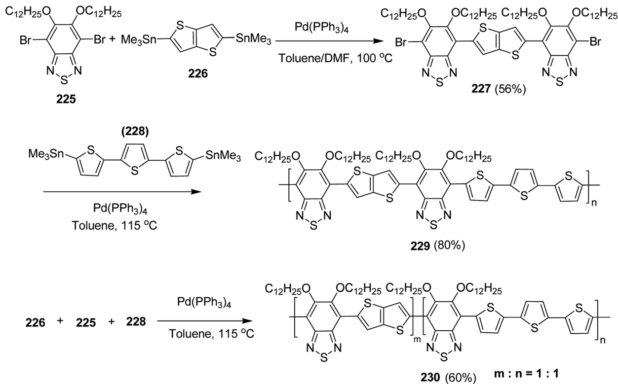
Scheme 77 Preparation of regioregular polymer 229 and regiorandom polymer 230.
