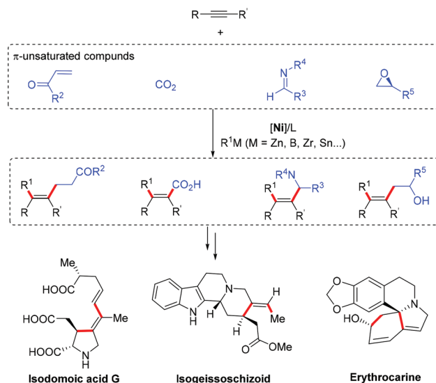
Scheme 15 Ni-Catalyzed reductive coupling of alkynes and various \pi -unsaturated compounds and synthetic applications.
