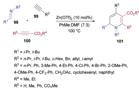
Scheme 22 Zn(OTf) 2 -catalyzed three-component synthesis of highly functionalized 1,6-dihydropyridines from aldimines and two alkynes.
