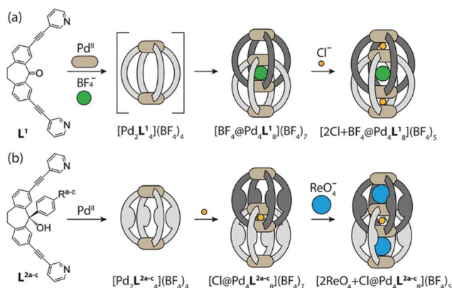
Fig. 16 Synthesis of interpenetrated dimer cage: (a) ([\text{Pd}_4\text{L}_8\text{-BF}_4]) with \text{BF}_4^- as a template anion and \text{Cl}^- anions in the outer pockets, (b) ([\text{Pd}_4\text{L}_8\text{-Cl}]) with \text{Cl}^- as a template anion and \text{ReO}_4^- in the outer pockets. Reproduced with permission from ref. 73. Copyright 2013, American Chemical Society.
