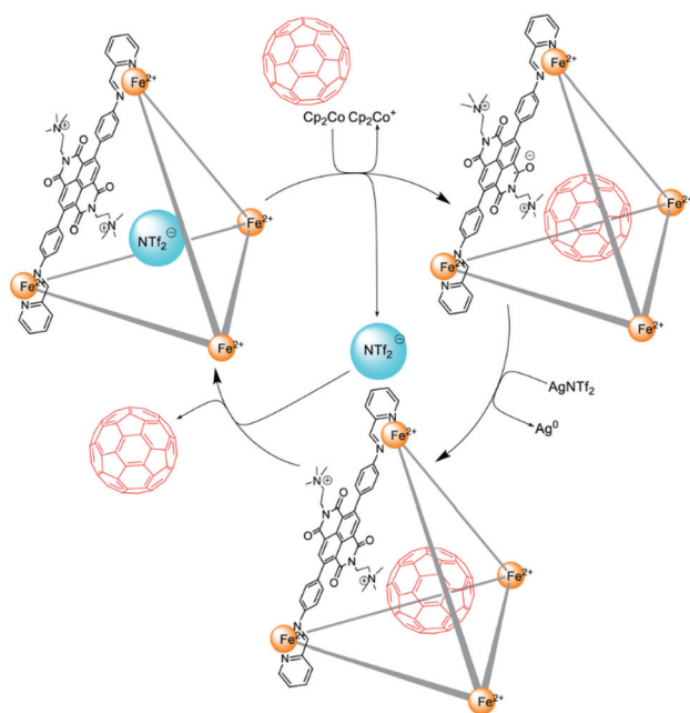
Fig. 5 The encapsulation and release of \text{C}_{60} within cage \text{II}^{\text{ve}}_{\text{Fe}} following reduction and subsequent re-oxidation. Reproduced with permission from ref. 50. Copyright 2020, the Royal Society of Chemistry.
