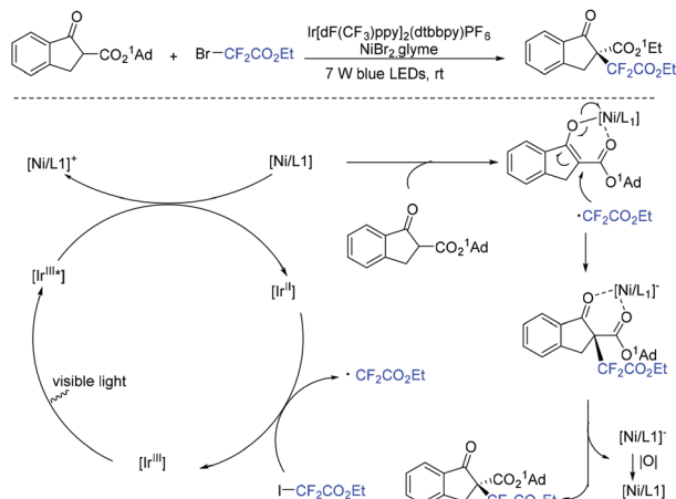
Scheme 103 The difluoroalkylation reactions of \beta -ketoesters.
