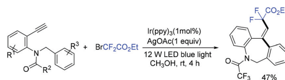
Scheme 62 The synthesis of substituted dibenzazepines catalyzed by \text{Ir(ppy)}_3 .
