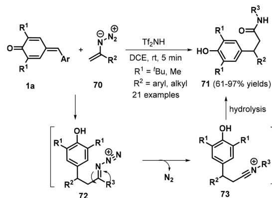
Scheme 16 Tf 2 NH-Catalyzed rearrangement of p -QMs.
