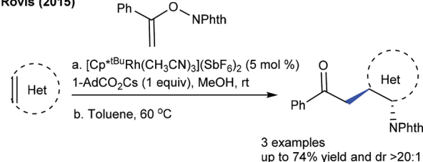
Scheme 42 syn -Carboamination of heterocyclic alkenes.
