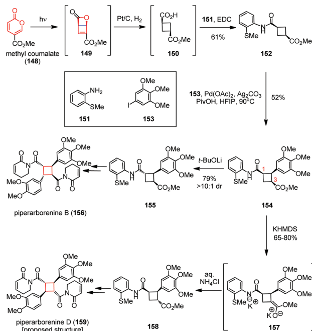
Scheme 22 4π electrocyclic ring closure in the total syntheses of piperaborenines.
