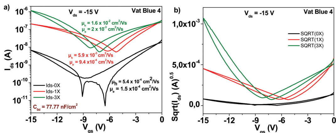
Fig. 8 (a) Comparison of OFET devices with three different purity grades of vat blue 4 semiconductor: unpurified (0x in graph legend), one time purified (1x in graph legend) and three times purified, respectively (3x in graph legend); (b) the \text{sqrt}(I_{ds}) vs. V_{gs} of the three purity grades presented in panel (a).
