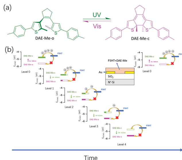
Fig. 17 (a) Chemical structure of the used DAE, in its open and closed form. (b) Middle: Structure illustration of the devices on a SiO 2 substrate. Schematic diagram of a multi-level storage device. With the increase of the 313 nm ultraviolet light irradiation time, the device gradually changed from level 0 to level 4, and then by 546 nm visible light irradiation, the device returned to level 0.
