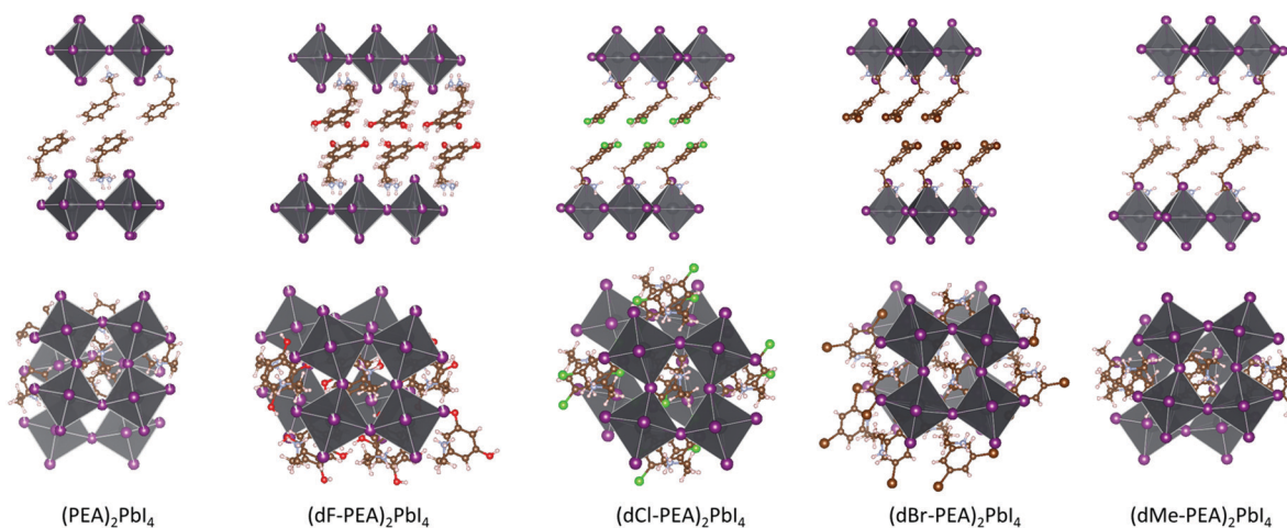
Fig. 2 Crystal structure of (\text{dY-PEA})_2\text{PbI}_4 , \text{Y} = \text{H}, \text{F}, \text{Cl}, \text{Br}, \text{Me} , viewed along the plane of the inorganic sheet and after +90^\circ rotation around the long in-layer axis. The structure of (\text{PEA})_2\text{PbI}_4 is taken from the literature. 34
