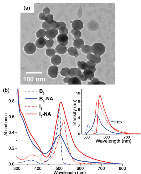
Fig. 5 (a) Transmission electron micrograph of I_6 -NA in water. (b) Absorption and (inset) fluorescence spectra of B_3 (6 \mu\text{M} ) and I_6 (4.5 \mu\text{M} ) in acetonitrile and B_3 -NA (10 \mu\text{g mL}^{-1} ) and I_6 -NA (10 \mu\text{g mL}^{-1} ) in water. The emission spectra were obtained by exciting the samples at the respective absorption maxima.
