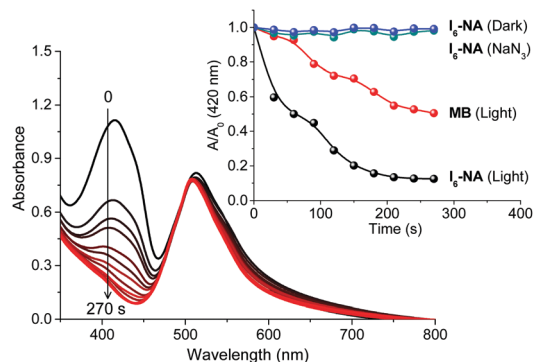
Fig. 6 Changes in the UV-Vis absorption spectrum of a mixture of 1,3-diphenylisobenzofuran (DPBF, 90 \mu\text{M} ) and I_6 -NA (10 \mu\text{g mL}^{-1} ) as a function of irradiation time in 20% ethanol-water. Inset shows the relative decrease in the absorption of DPBF at 420 nm in the presence of I_6 -NA or methylene blue (MB) under different experimental conditions.
