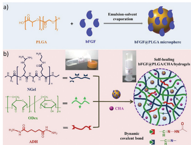
Fig. 24 Schematic presentation of (a) fabrication of bFGF@PLGA microspheres; (b) preparation of bFGF@PLGA/CHA/hydrogels through formation of dynamic imine/hydrazone bonds between aminated gelatin (NGel), adipic acid dihydrazide (ADH) and oxidized dextran (ODex), and further encapsulation of bFGF@PLGA microspheres and drug chlorhexidine acetate (CHA), leading to sequential release of CHA during wound healing. 11 Copyright 2019 Elsevier.
