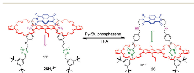
Fig. 26 Double-leg donor–acceptor molecular elevator 26 .
