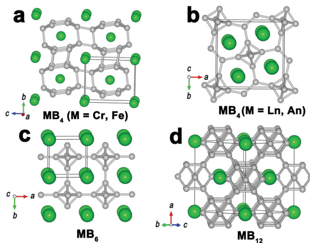
Fig. 6 Crystal structures of (a) MB_4 ( M = Cr, Fe ); (b) MB_4 ( M = Ln, An ); (c) MB_6 ( M = K, Ca, Sr, Ba, Y, La, Ce, Pr, Nd, Sm, Eu, Gd, Tb, Dy, Ho, Er, Tm ); (d) MB_{12} ( M = Zr, Hf, Y, Gd, Tb, Dy, Ho, Er, Tm, Yb, Lu, Th, U and Pu ). Metal atoms and boron atoms are in green and grey, respectively.
