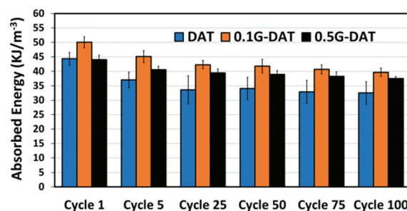
Fig. 7 100 cycle fatigue test for (G)-DAT hydrogels.
