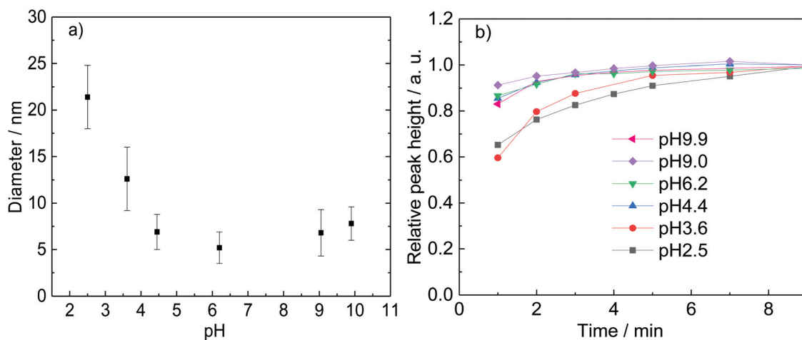
Fig. 9 Effect of pH on a. Au NP sizes (the error bars represent the standard deviation) and b. rate of formation. Conditions: [AuCl]: 0.25 mM, [\text{DC}^{2-}] : 5 mM, [citrate]: 5 mM, 80 °C, time: 7 min–13 min.
