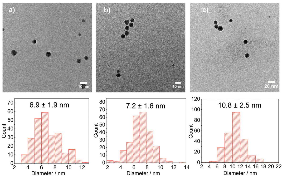
Fig. 8 Representative TEM images and particle size distribution of Au NPs synthesised using AuCl as precursor with a \text{DC}^{2-} : Au molar ratio of a. 20 : 1, b. 10 : 1 and c. 1 : 1. Conditions: [AuCl]: 0.25 mM, [citrate]: 5 mM, pH: 4.4, 80 °C, time: 7 min–11 min.
