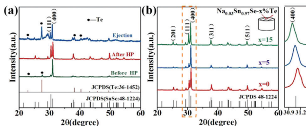
Fig. 1 (a) Powder XRD patterns for \text{Na}_{0.03}\text{Sn}_{0.97}\text{Se}-5\% \text{Te} in different processes; (b) bulk XRD patterns for \text{Na}_{0.03}\text{Sn}_{0.97}\text{Se}-x\% \text{Te} ( x = 0, 5 and 15 ) measured on the surface perpendicular to the pressing direction.
