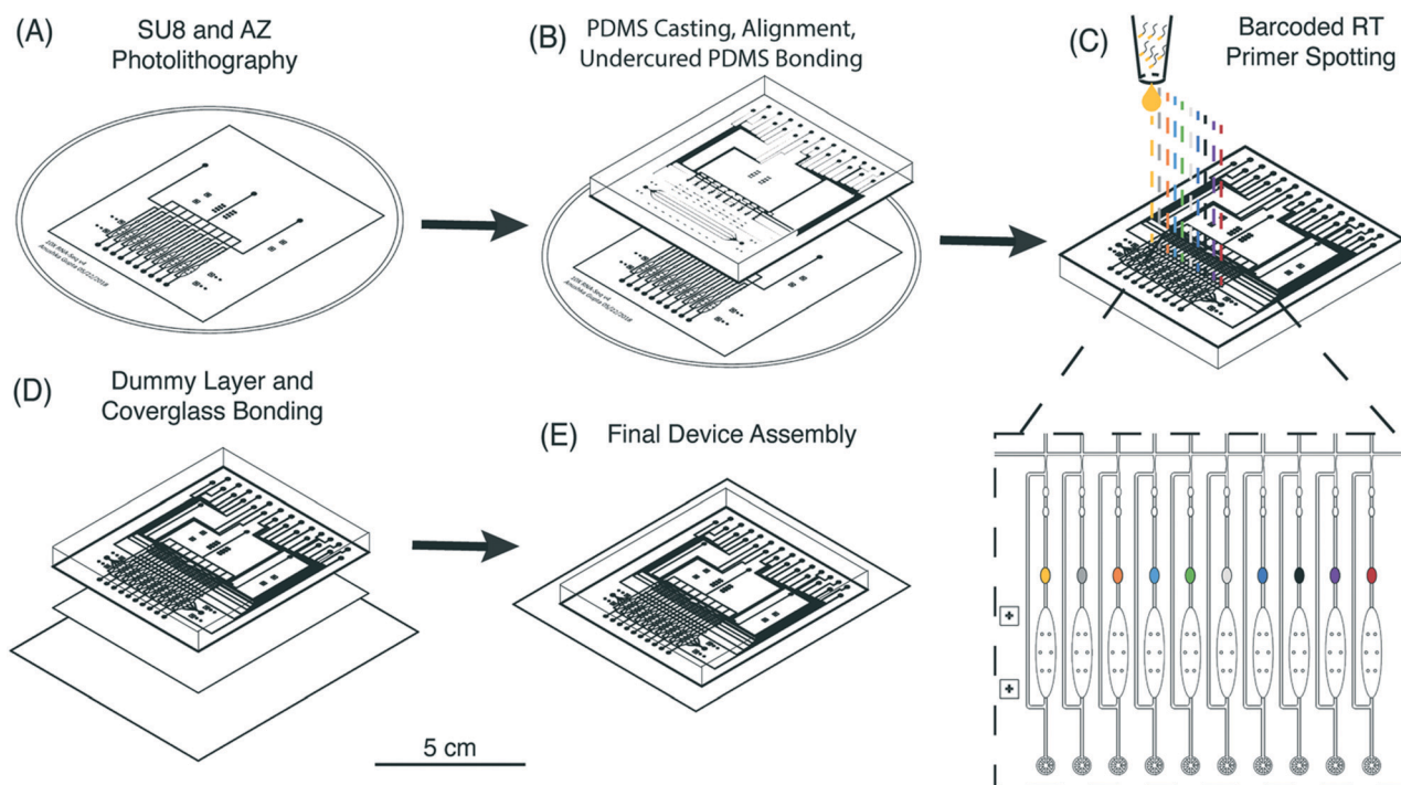
Fig. 2 Fabrication of \mu CB-seq devices with barcoded RT primer spotting. (A) Photolithographic patterning of control and flow layers. (B) Diagram of PDMS casting and undercured PDMS bonding between the control and flow layers. (C) Detailed diagram of barcoded RT primer spotting. Unique primers are delivered to each lysis module and dried before the device is closed (D) by bonding to a PDMS dummy layer. (E) PDMS devices are then plasma bonded to a coverslip for final assembly. The scale bar refers to the panels (A) to (E).
