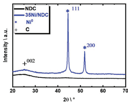
Fig. 5 XRD patterns recorded for the parent NDC and freshly reduced 35Ni/NDC.
